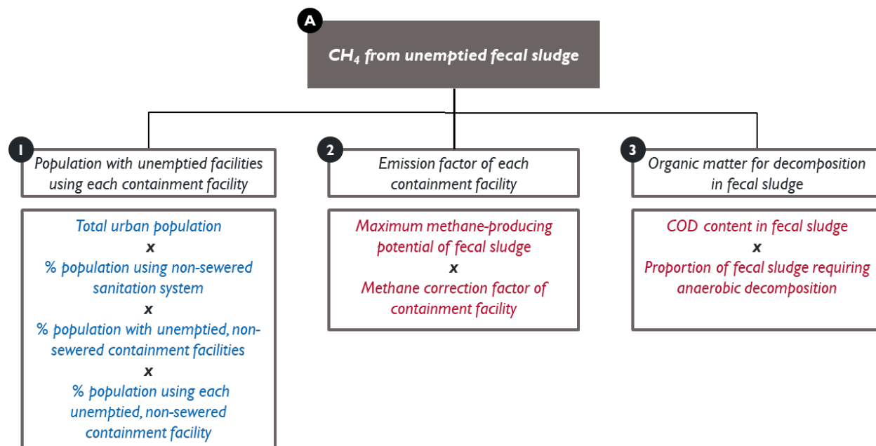
Figure 23. Inputs required for calculating emissions from each unemptied containment facility
