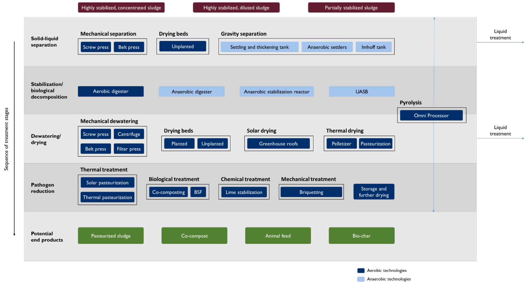
Figure 11. Technology processes and choices for fecal sludge treatment plants
