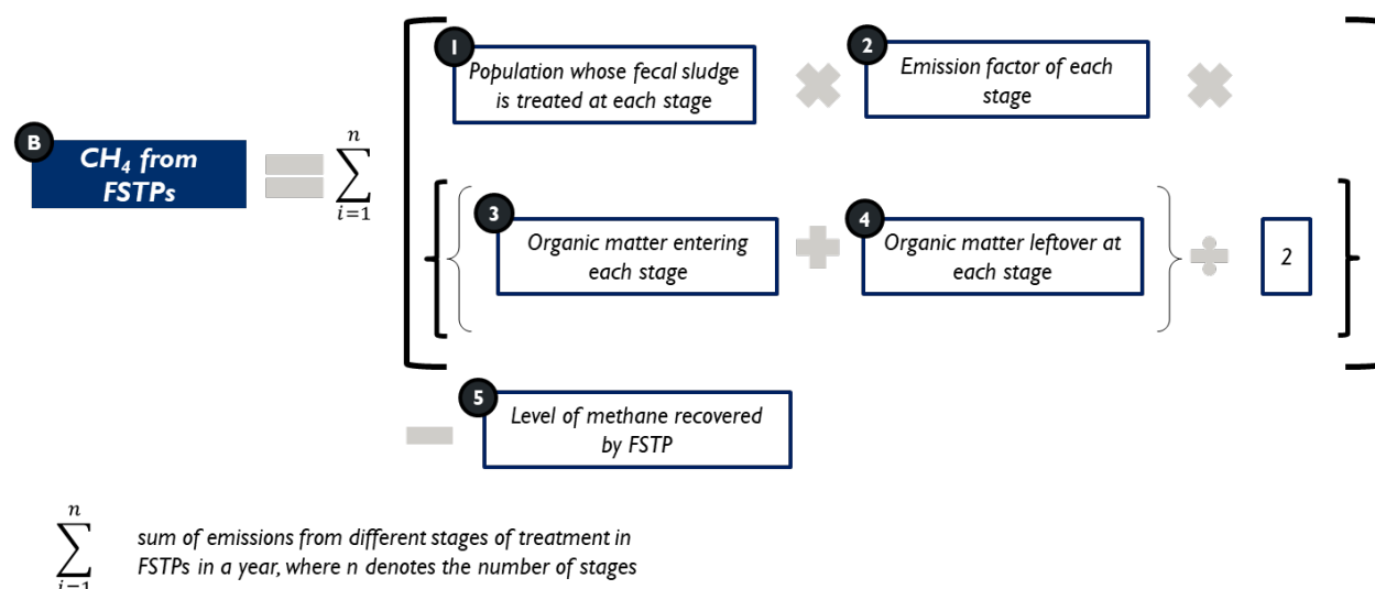
Figure 24. Equation to calculate emissions from an FSTP
